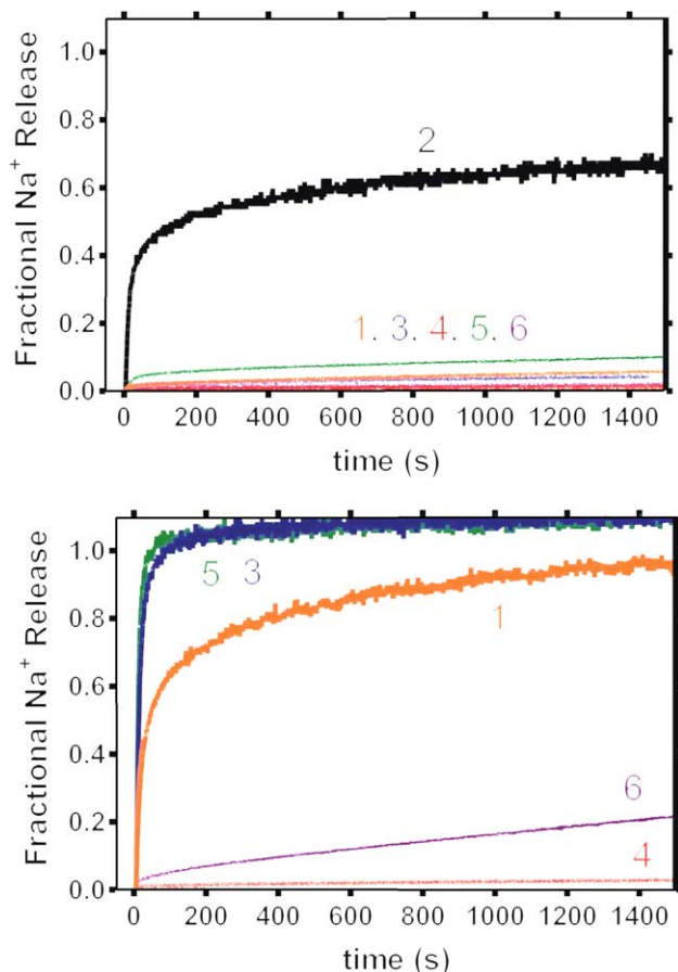
Figure 2. Comparison of \text{Na}^+ -release activity from liposomes mediated by 1–6 at concentrations of 12 \mu\text{M} (upper panel) and 60 \mu\text{M} .
