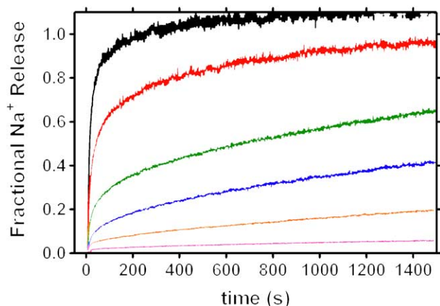
Figure 1. Fractional sodium ion release from phospholipid vesicles mediated by 1 .
